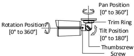
Figure 2-10 3-Axis Adjustment
