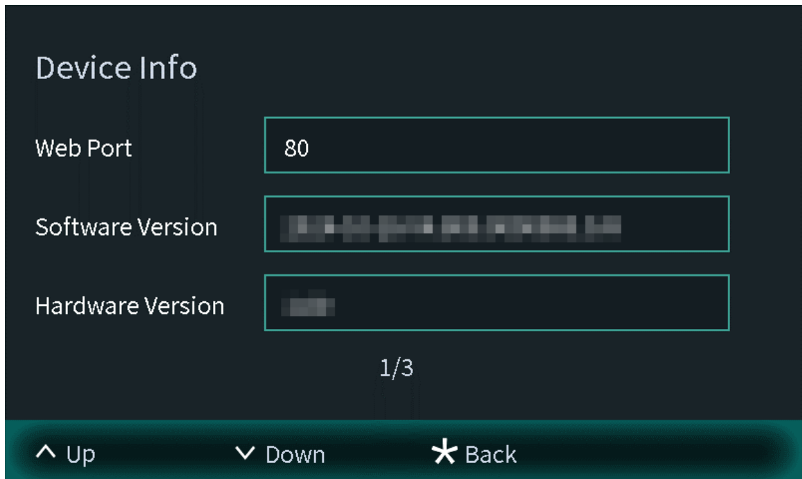
Figure 2-25 Device information (2)
