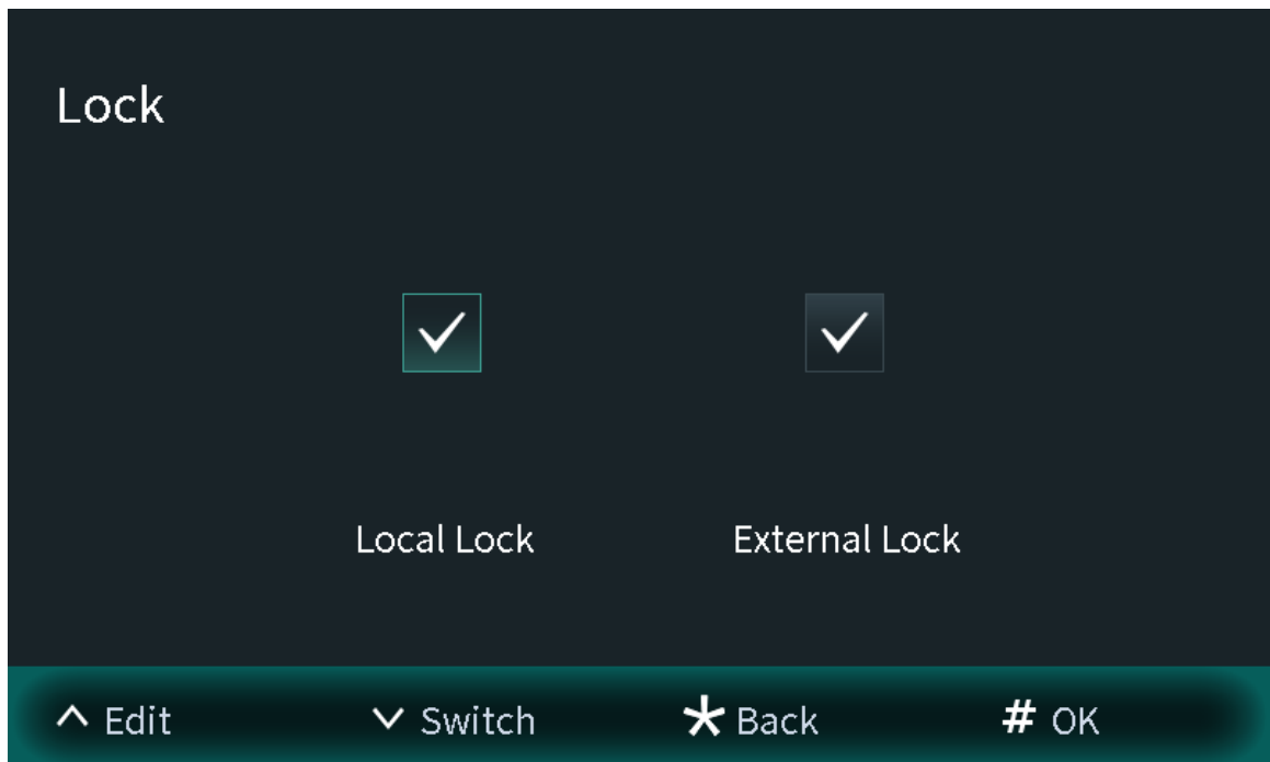
Figure 2-19 Lock
