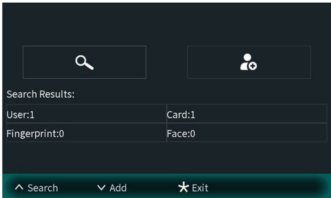
Figure 2-23 Search result
