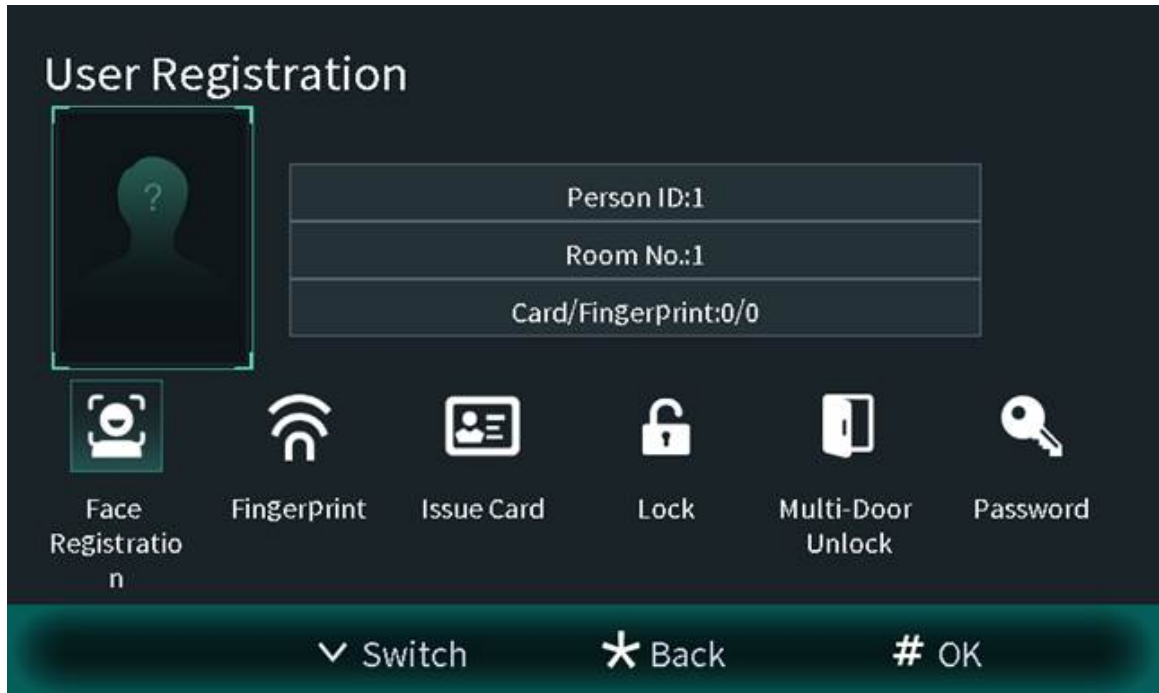
Figure 2-13 Face registration
