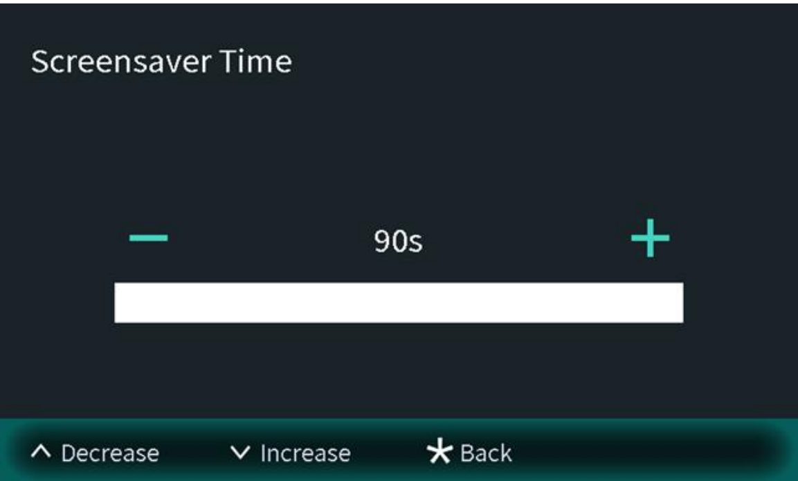
Figure 2-9 Screensaver time
