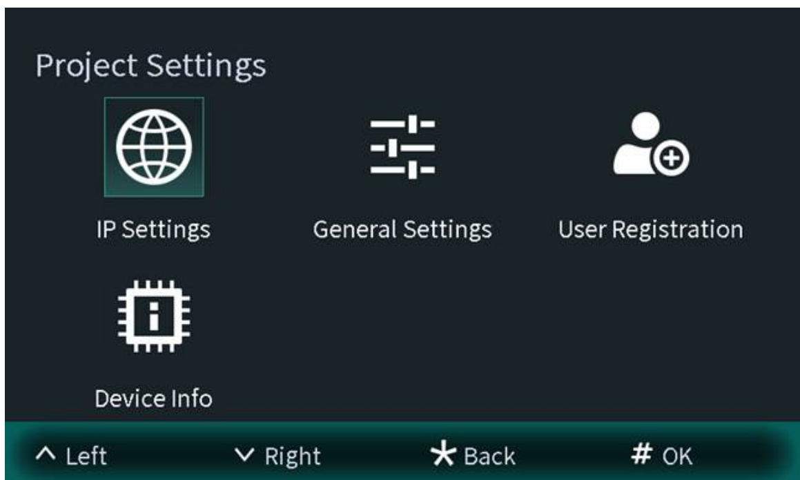
Figure 2-4 Engineering setting
