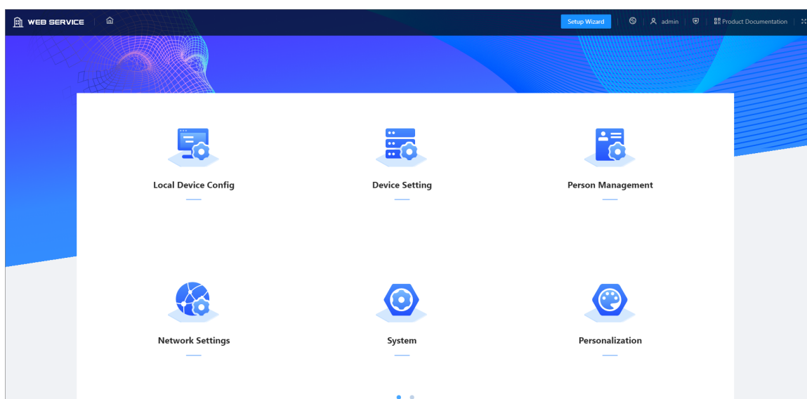
Figure 3-2 Home page
