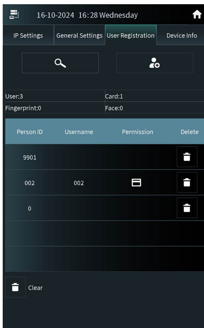
Figure 2-41 User list
