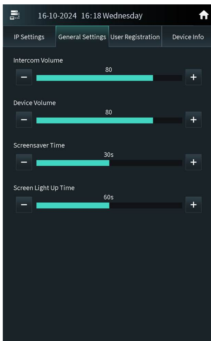
Figure 2-30 General settings
