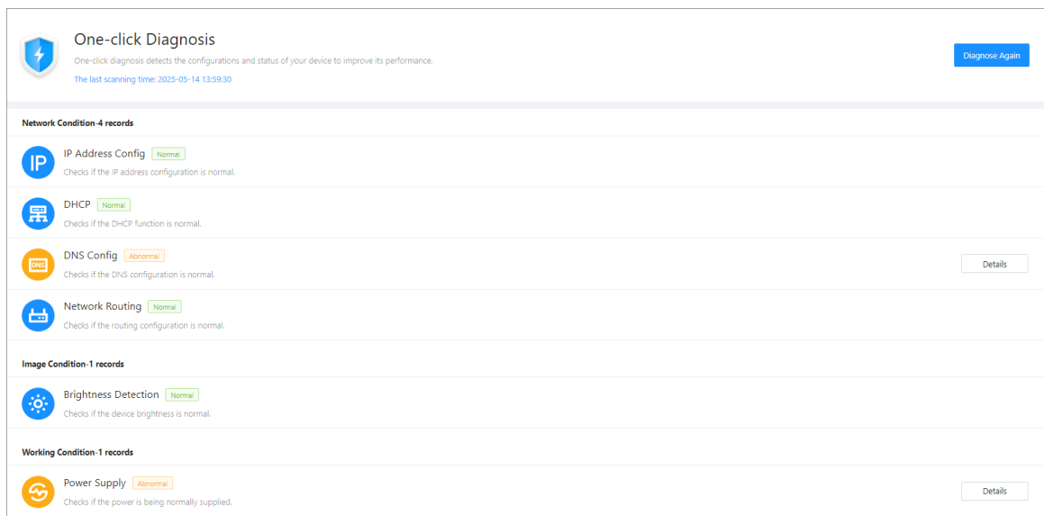
Figure 3-70 One-click diagnosis
