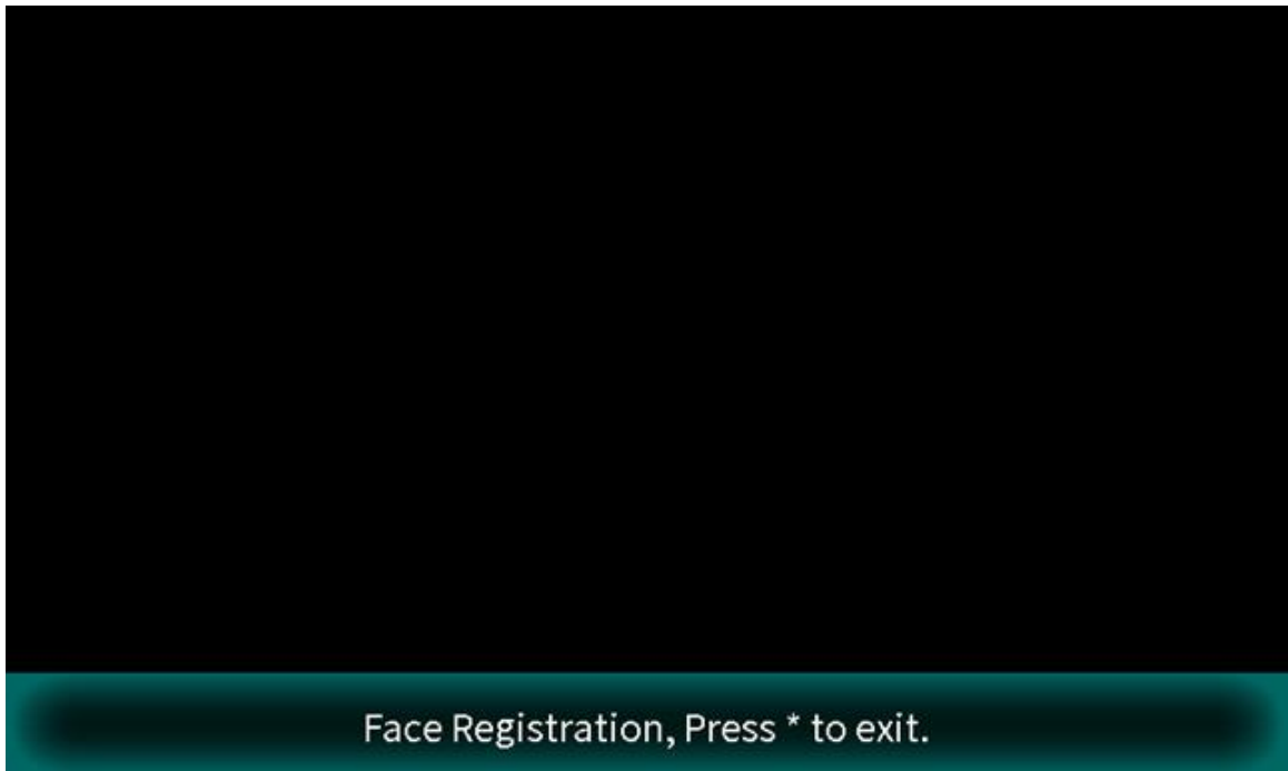
Figure 2-14 Face registration
