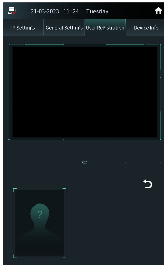
Figure 2-34 Face registration
