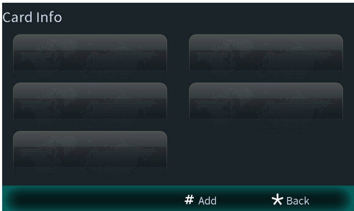
Figure 2-15 Card information
