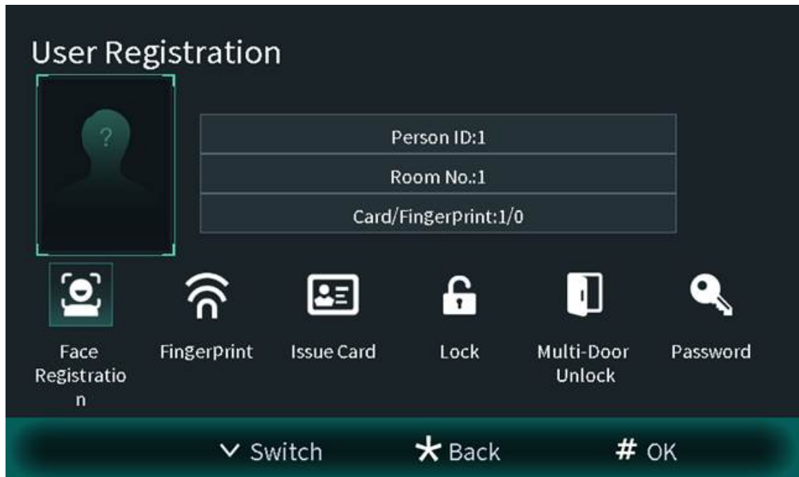
Figure 2-22 User information
