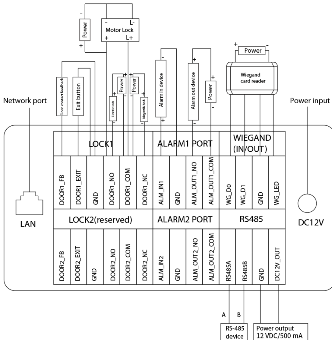
Figure 1-7 Cable connection
